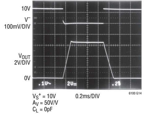
Step Response at V_{\text{SENSE}} = 0\text{V} to 130\text{mV}
