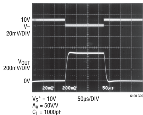
Step Response at V_{\text{SENSE}} = 0\text{V} to 10\text{mV}
