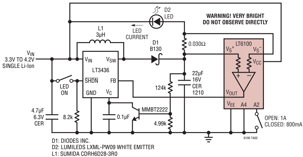
800mA/1A White LED Current Regulator
