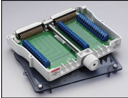
Model 3731-ST: Screw Terminal Block.
