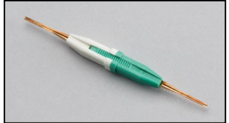
Model 3791-CIT: Contact insertion and extraction tool for assembly and maintenance of Series 3700A D-sub Connector kits.
