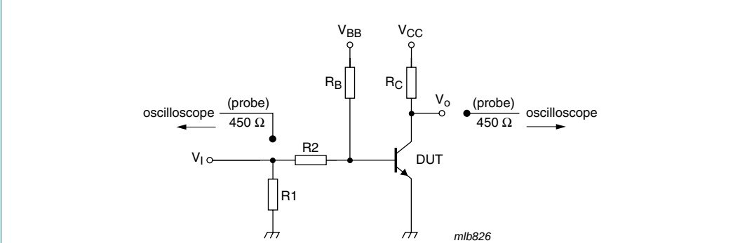
Fig 22. TR1 (NPN): Test circuit for switching times
