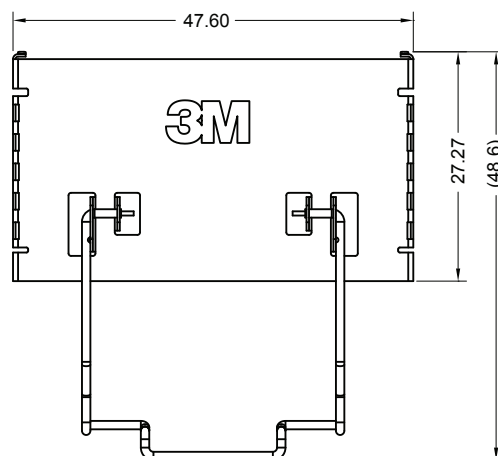
LATCHING RETAINER
