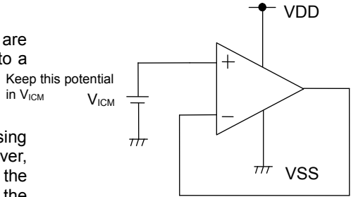
Figure 79. Example of Application Circuit for Unused Op-amp
