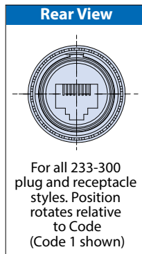
00, D0, CM - Wall Mount Receptacle
