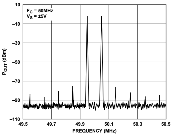
Figure 19. Intermodulation Distortion
