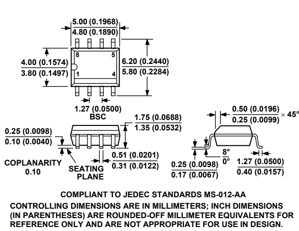
Figure 50. 8-Lead Standard Small Outline Package [SOIC] (R-8) Dimensions shown in millimeters and (inches)
