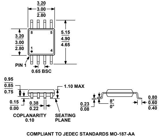
Figure 51. 8-Lead Mini Small Outline Package [MSOP] (RM-8) Dimensions shown in millimeters
