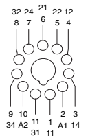
Terminal Arrangement
