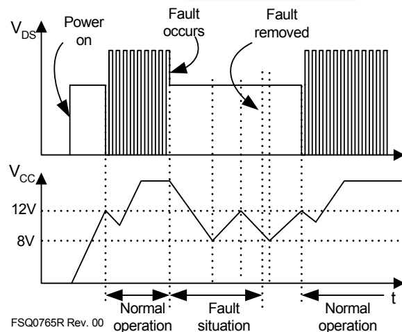
Figure 37. Auto-Restart Protection Waveforms
