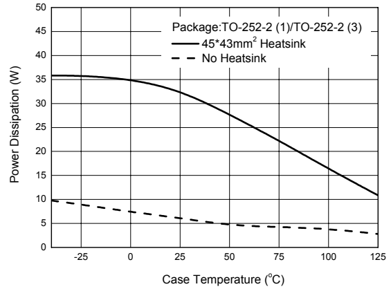
Figure 21. Power Dissipation vs. Case Temperature
