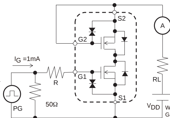
Test Circuit 8
