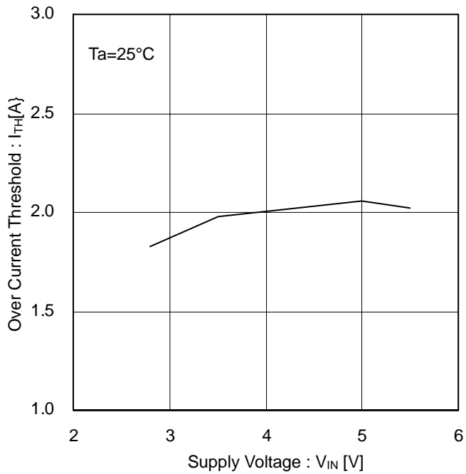
Figure 14. Over-Current Threshold
