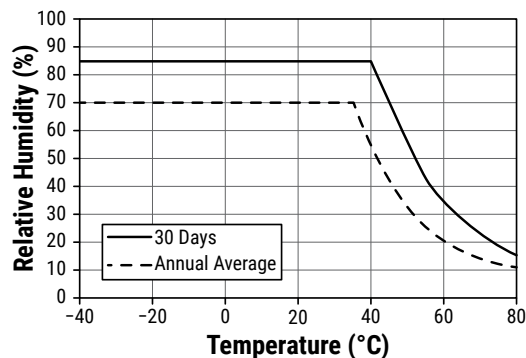
Maximum Humidity in Storage Conditions
