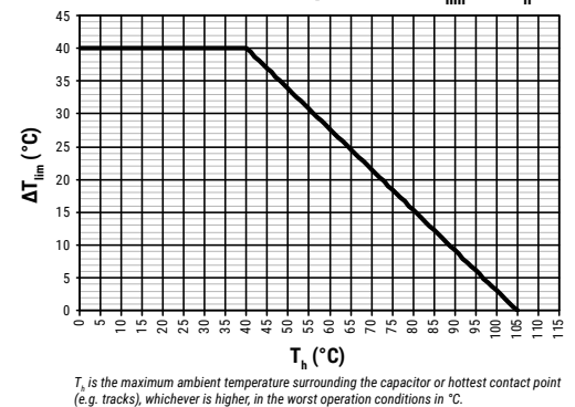
Maximum Overtemperature \Delta T_{lim} vs. T_h
