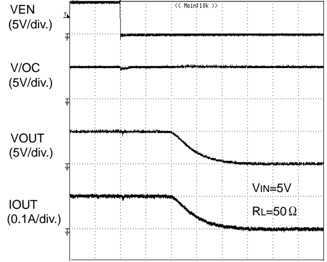
Figure 33. Output fall characteristic
