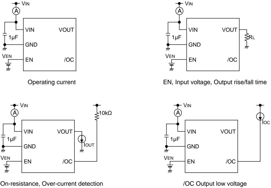
Figure 4. Measurement circuit
