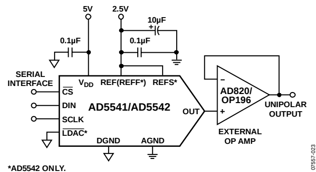
Figure 23. Unipolar Output
