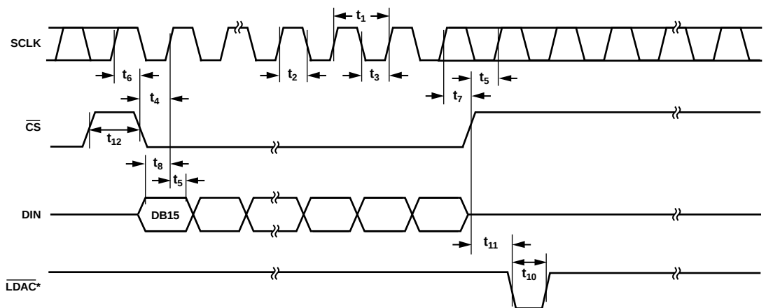
Figure 3. Timing Diagram
