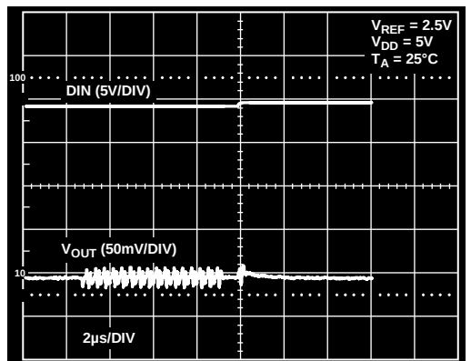
Figure 18. Digital Feedthrough
