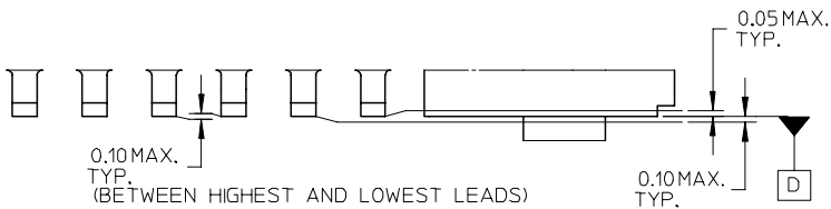
DETAIL 1
