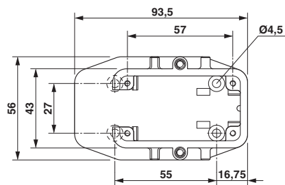
Dimensional drawing top view
