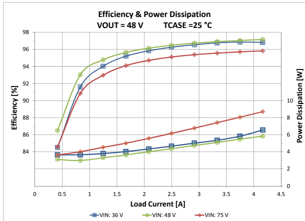
Figure 8: Total efficiency and power dissipation vs. V IN and I OUT V OUT = 48 V, T CASE = 25 °C
