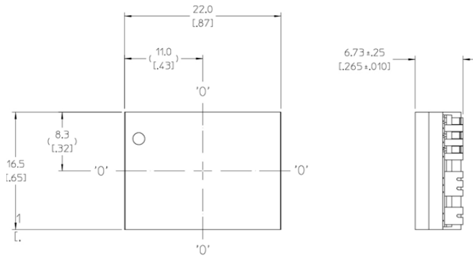
TOP VIEW (COMPONENT SIDE)
