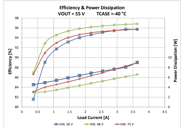
Figure 10: Total efficiency and power dissipation vs. V IN and I OUT V OUT = 55 V, T CASE = -40 °C
