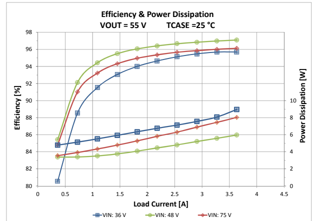
Figure 11: Total efficiency and power dissipation vs. V IN and I OUT V OUT = 55 V, T CASE = 25 °C
