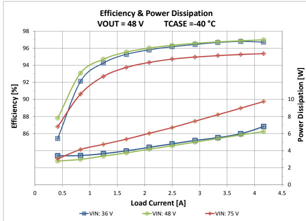
Figure 7: Total efficiency and power dissipation vs. V IN and I OUT V OUT = 48 V, T CASE = -40 °C
