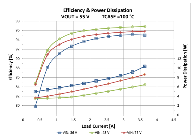
Figure 12: Total efficiency and power dissipation vs. V IN and I OUT V OUT = 55 V, T CASE = 100 °C
