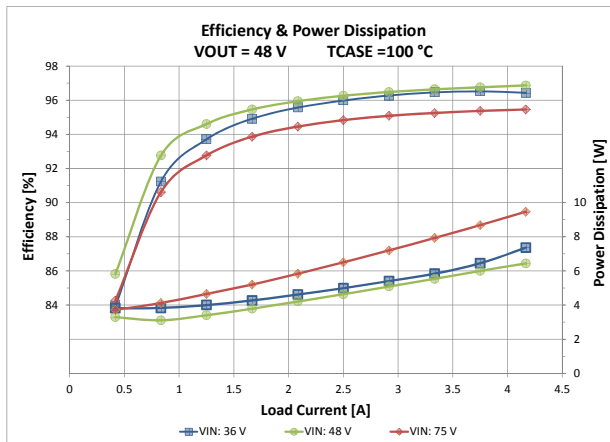
Figure 9: Total efficiency and power dissipation vs. V IN and I OUT V OUT = 48 V, T CASE = 100 °C
