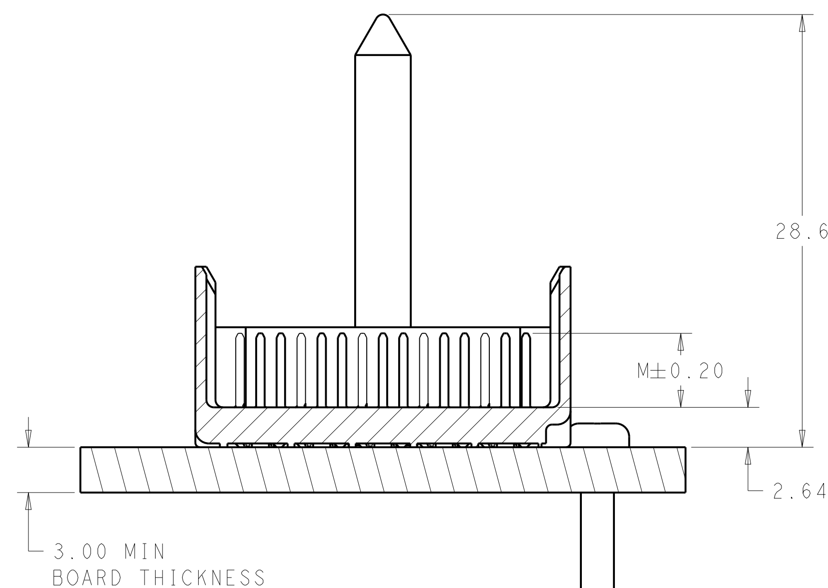
SECTION Z-Z
