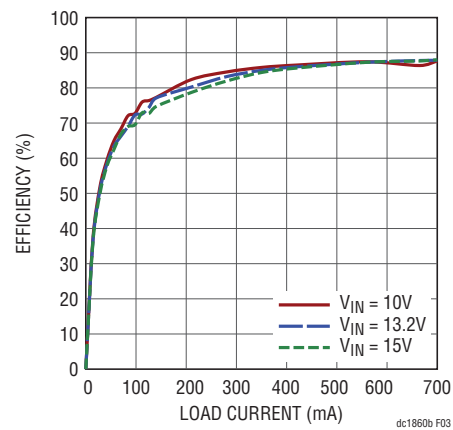
Figure 3. Typical Efficiency Curve, (TA = 25°C)
