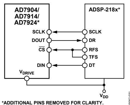
Figure 31. Interfacing to the ADSP-218x
