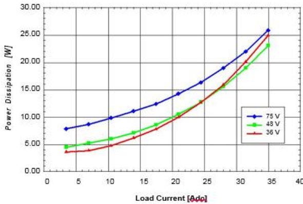
Figure 30. Power dissipation vs. load current and input voltage for converter w/o baseplate mounted vertically with air flowing from pin 3 to pin 1 at a rate of 300 LFM (1.5 m/s) and T_a = 25\text{ }^\circ\text{C} .
