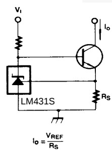
Figure 9. Constant-Current Sink
