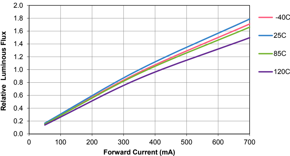
Figure 32. LUXEON F Cool White relative luminous flux vs. forward current MP [1] .
