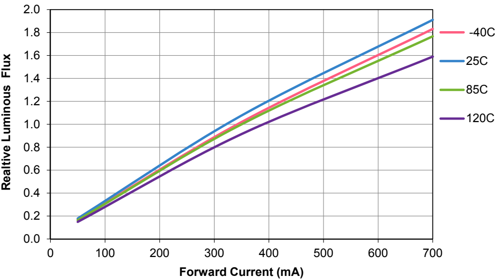
Figure 31. LUXEON F Cool White relative luminous flux vs. forward current DC.
