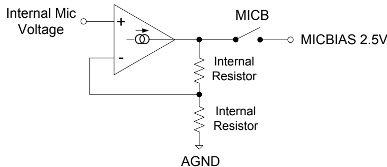
Figure 13. Mic Bias
