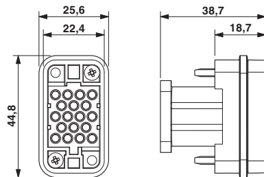
HC-COM-17-ESTC dimensional drawing
