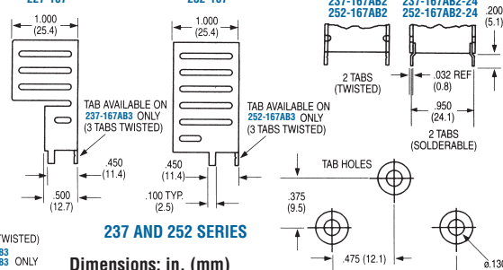
237 AND 252 SERIES Dimensions: in. (mm)
