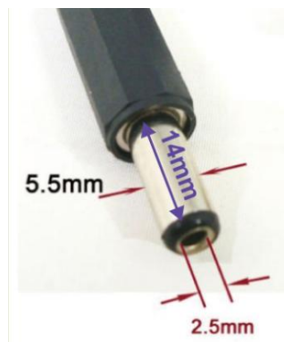
Figure 2-5 DC-Plug Specification
