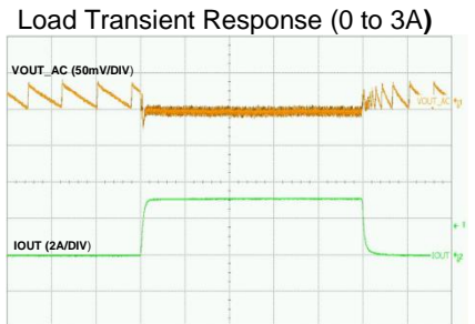
Time-100μs/div
