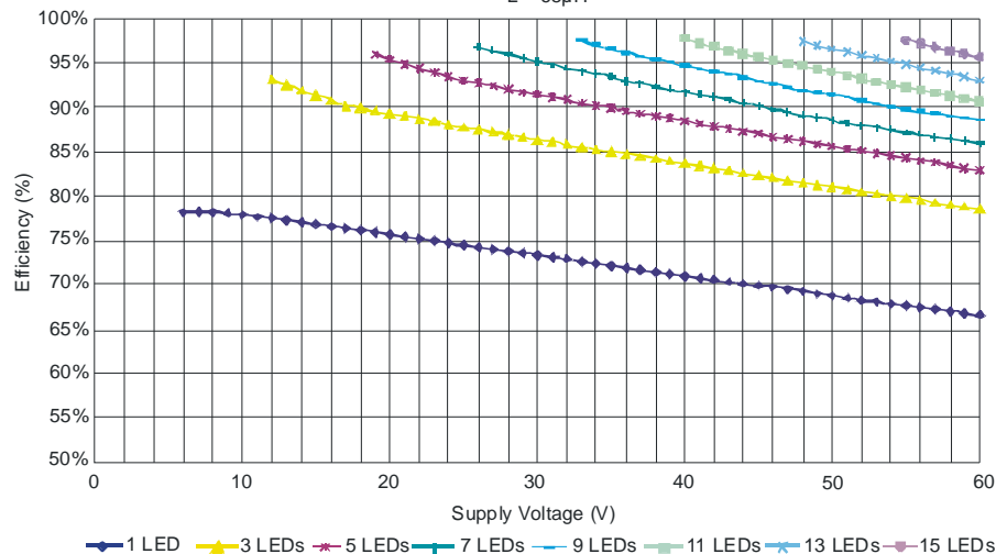
ZXLD1356 Efficiency L = 68 \mu H
