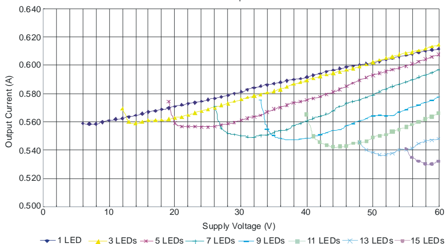
ZXLD1356 Output Current L = 68 \mu H
