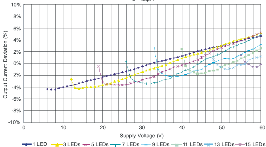
ZXLD1356 Output Current Deviation (Normalized) L = 68 \mu H
