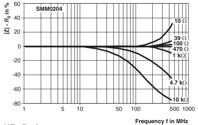
HF - Performance
