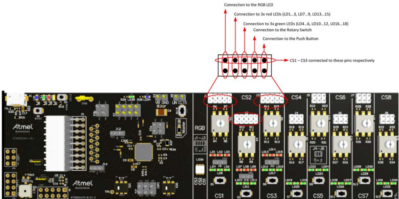
Figure 3-9. Jumpers JP1...3
