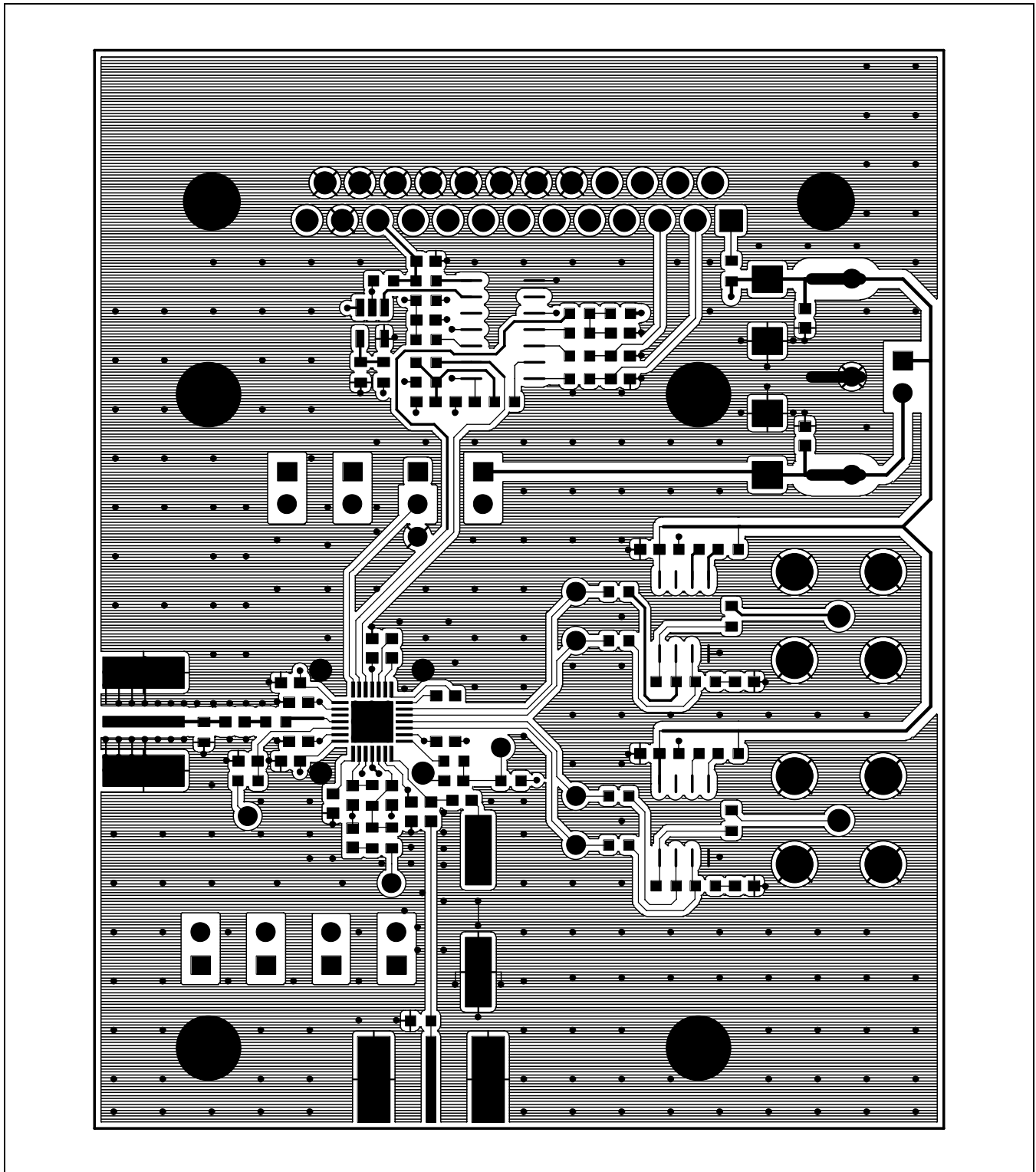
Figure 3. MAX2120 EV Kit PCB Layout—Top
