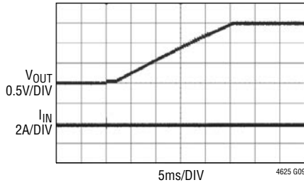
Start-Up with No Load Current
