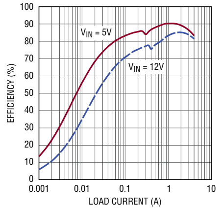
DCM Mode Efficiency, V OUT = 1.5V
