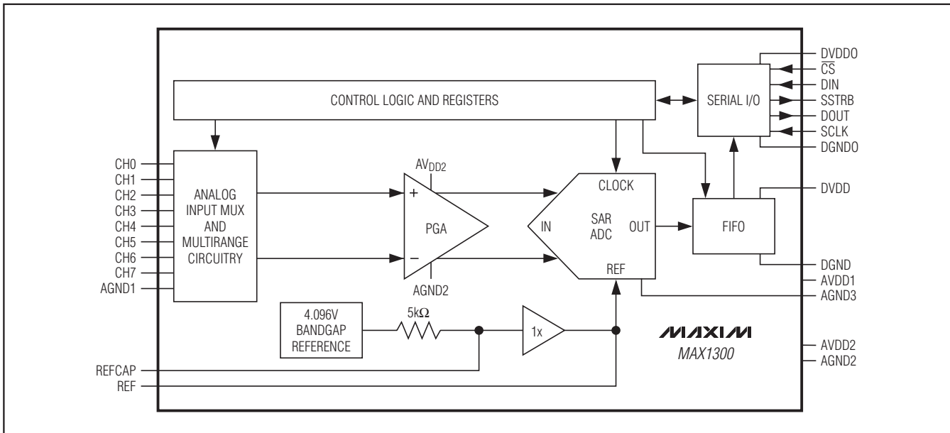
Block Diagram
