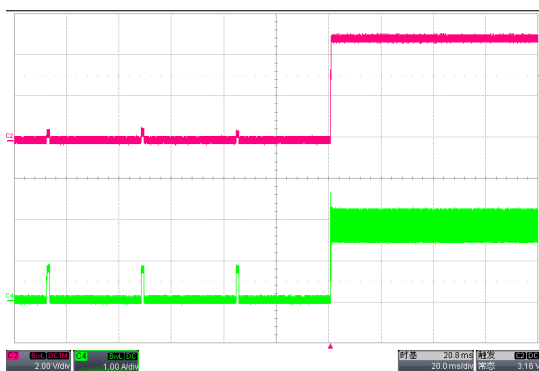
Figure 16 V_{OUT} Short Recovery ( I_O = 1\text{A} ) (CH2: V_{OUT} ; CH3: IL)
