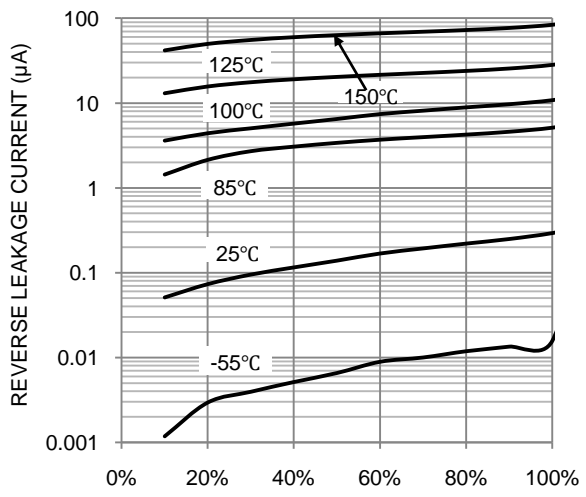
V_R , PERCENTAGE RATED PEAK REVERSE VOLTAGE (%) Fig.5 Typical Reverse Characteristics
