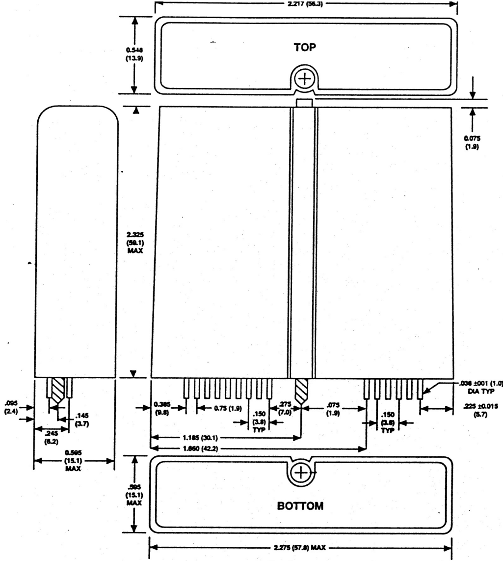
Figure 5. Outline Dimensions
