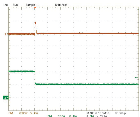
Step Load Transient Response (Vin=5.0V, Vout=3.3V, Cload=94μF, Iout=20A to 10A) Trace 1=Vout, 200 mV/div, Trace 4=Iout, 10A/div.
