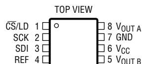
MS8 PACKAGE 8-LEAD PLASTIC MSOP
