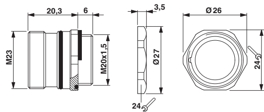
Dimensional drawing
