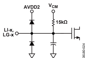
Figure 30. Equivalent LNA Input Circuit
