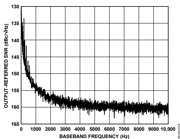
Figure 28. Output-Referred SNR vs. Baseband Frequency
