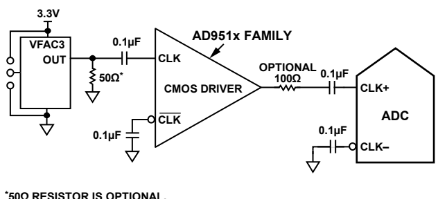
Figure 67. Single-Ended 3.3 V CMOS Sample Clock
