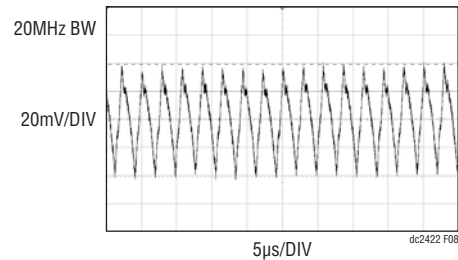
Figure 8. DC2422A-A V OUT1 Voltage Ripple at V IN = 36V
