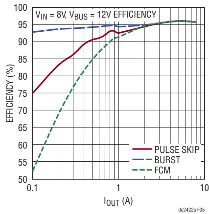
Figure 5. DC2422A-C V BUS Typical Efficiency vs Load Current
