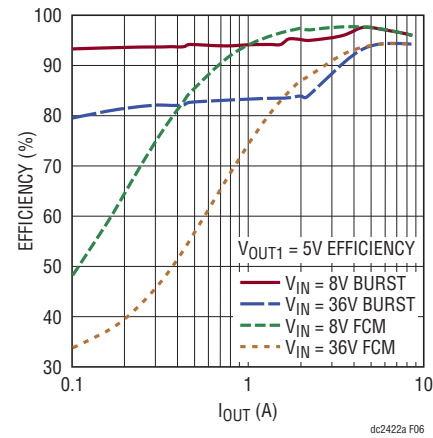
Figure 6. DC2422A-C V OUT1 Typical Efficiency vs Load Current
