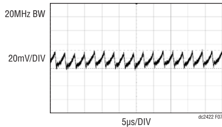
Figure 7. DC2422A-A V OUT1 Voltage Ripple at V IN = 8V
