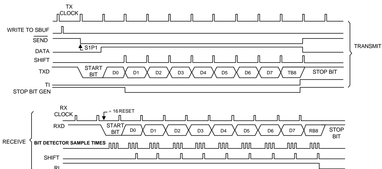
Figure 12. Serial Port Mode 3
