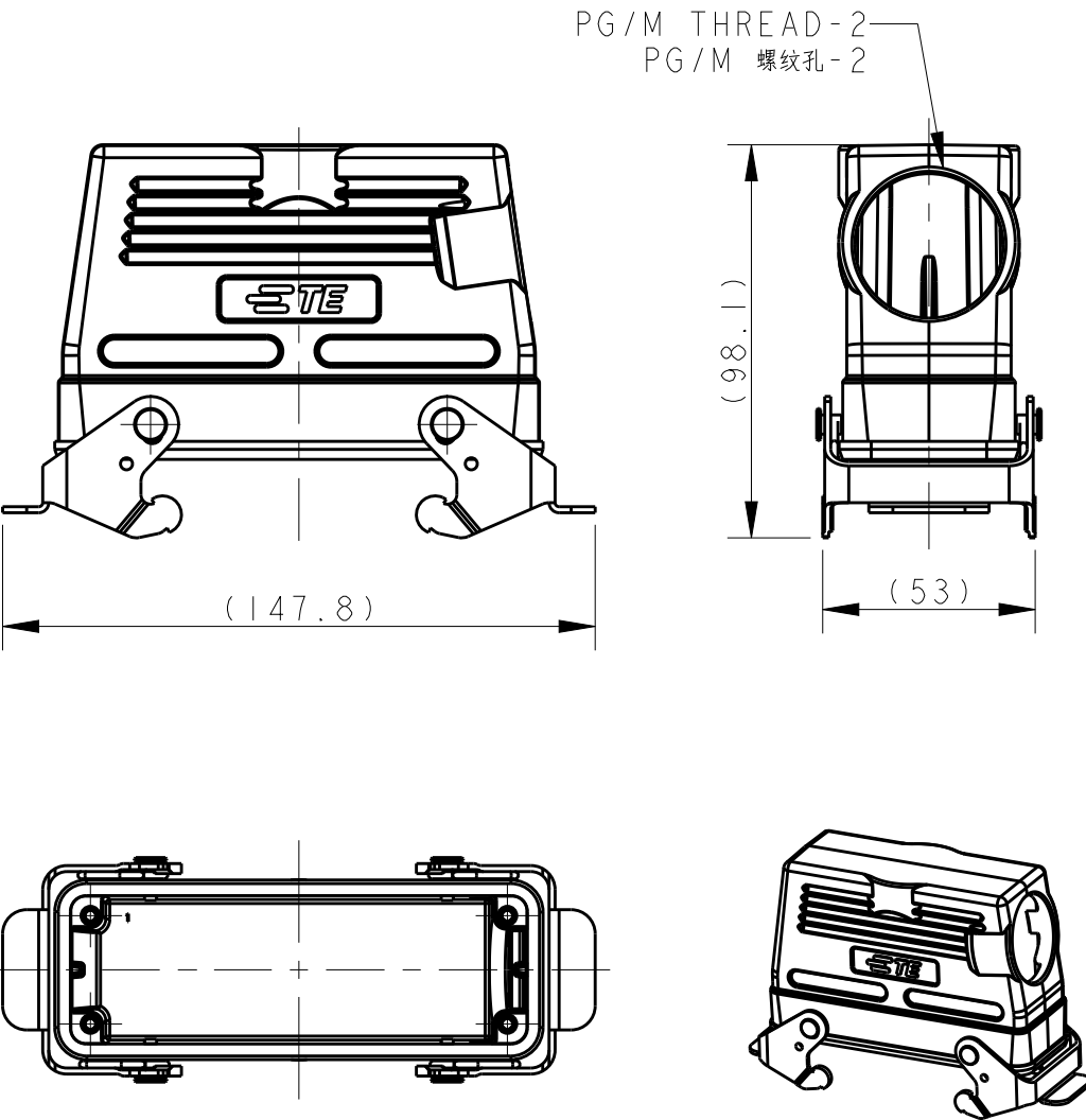
TYPE 7: HIGH CONSTRUCTION + METAL DOUBLE LOCKING + SIDE ENTRY, OTHER SPEC REFER TO TYPE 4 类型7：高结构壳体+彩锌双扣+侧出进线孔，其他规格参照类型4
