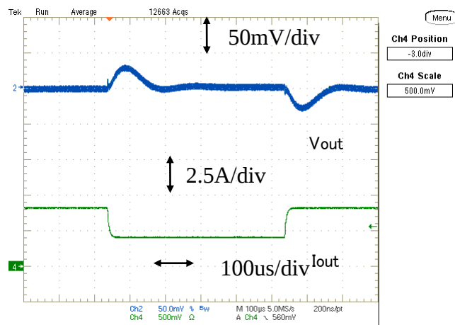
Fig. 12-1b. Load Transient Response ( C_{out}: 2000\mu F )
