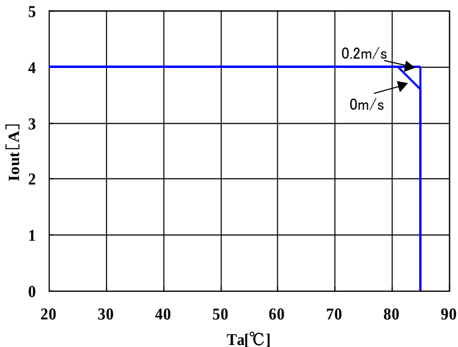
MPDTY321S ( V_{in}=4.5\sim 5.5V , V_{out}=0.8\sim 3.3V , Air Flow: 0\sim 0.2m/s )
