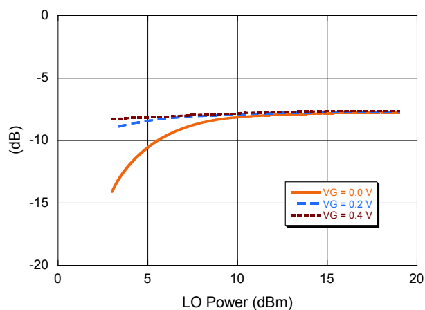
M \times N Spurious Rejection at IF Port (dBc IF)
