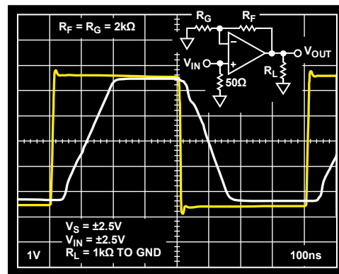
Figure 45. Overdrive Recovery
