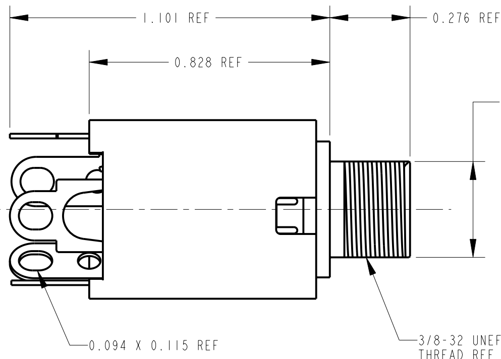
SOLDER TERMINAL OPTION
